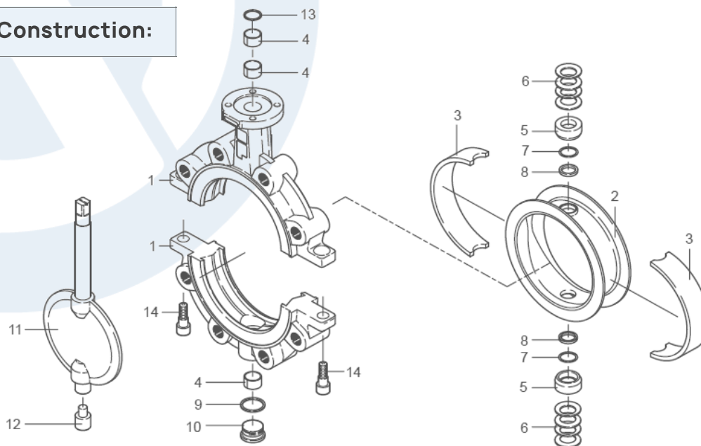
PTFE-lined butterfly valve DN 80 - DN 200
